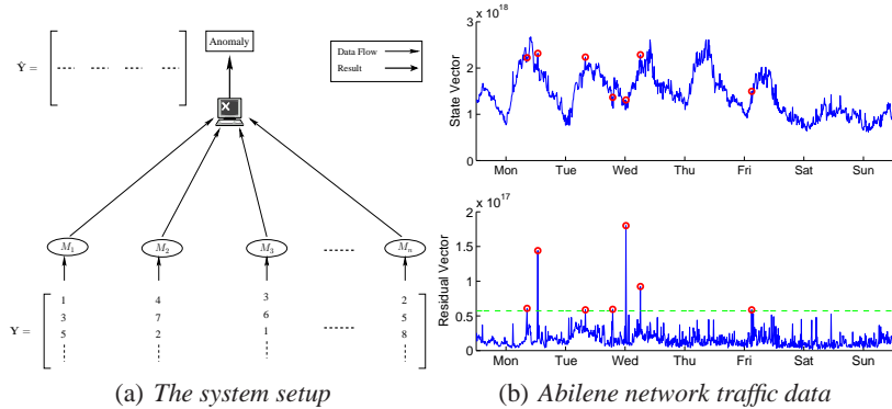
Figure 1: (a) The distributed monitoring system; (b) Data sample ( \|y\|^2 ) collected over one week (top); its projection in residual subspace (bottom). Dashed line represents a threshold for anomaly detection.
