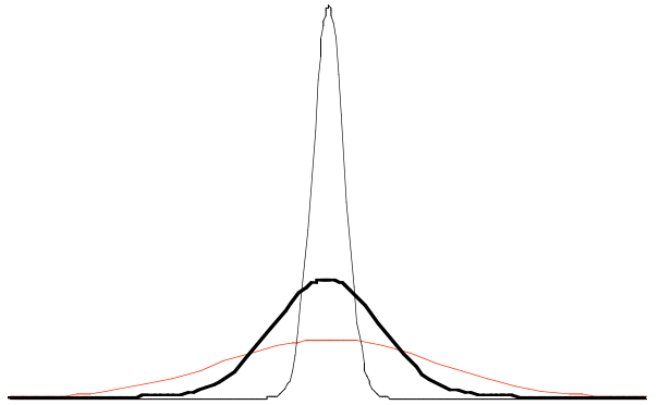
Figure 17 In Mediocristan, as your sample size increases, the observed average will present itself with less and less dispersion –as you can see, the distribution will be narrower and narrower. This is, in a nutshell, how EVERYTHING in statistical theory works (or is supposed to work). Uncertainty in Mediocristan vanishes under averaging. This illustrates the “law of large numbers”.
