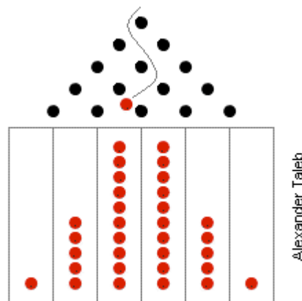
Figure 19- The Quincunx- The pinball machine. You drop balls that, at every step, randomly fall right or left. Above is the most probable scenario. It greatly resemble the Bell Curve (a. k. a. Gaussian distribution)
