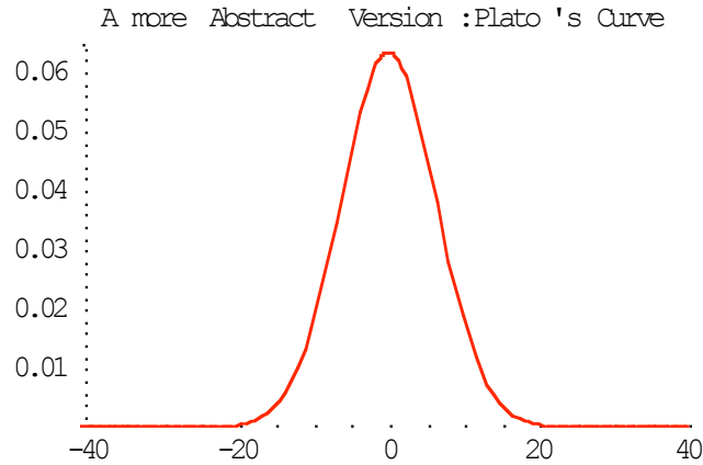
Figure 21 An infinite number of tosses
