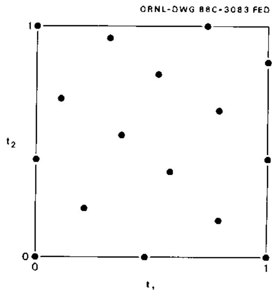
FIG. 1. Algorithmic-generated design: 16 runs, 2 inputs. Source: Figure 9, Currin, Mitchell, Morris and Ylvisaker (1988).
