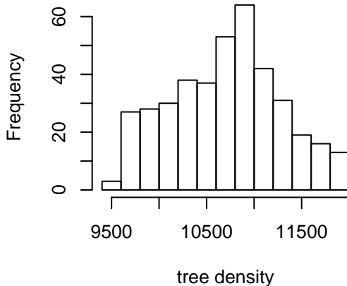
Tree Density at High Soil Moisture
