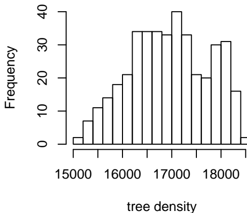
Tree Density at Low Soil Moisture
