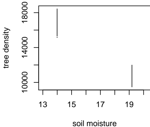
Yearly Density as function of input Soil Moisture
