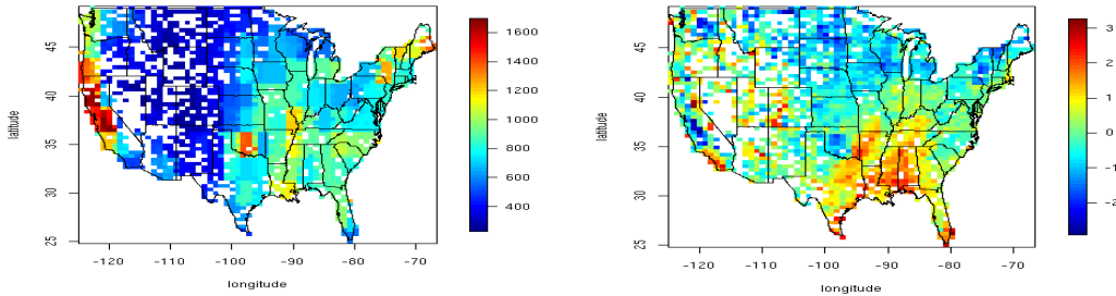
FIG 4. Simple Regression Model Including Elevation: Fitted return values (left) and residuals (right) from the regression model \text{Log}(\text{Point}) \sim \text{Grid} + \text{Elevation} using the NCEP grid cell data.
