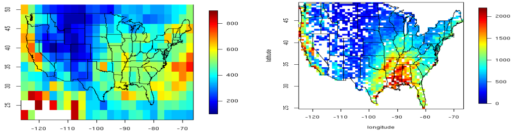
FIG 1. NCEP Grid and NCDC Station Return Levels: One-hundred-year return values, in tenths of a millimeter, computed for each grid cell in the NCEP data (left frame) and for each station from the NCDC data (right frame).
