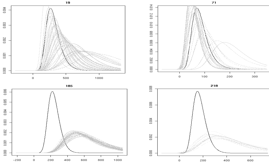
FIG 2. Densities: Solid black curves indicate the fitted GEV densities for four grid cells from the reanalysis (NCEP) grid data. San Francisco coast (top left): Latitude 37.5, Longitude -122.5; Montana (top right): Latitude 47.5, Longitude -112.5; Alabama (bottom left): Latitude 32.5, Longitude -87.5; and Key Largo, FL (bottom right): Latitude 25, Longitude -80. Dotted grey curves indicate the fitted densities from each NCDC station within the grid cells.
