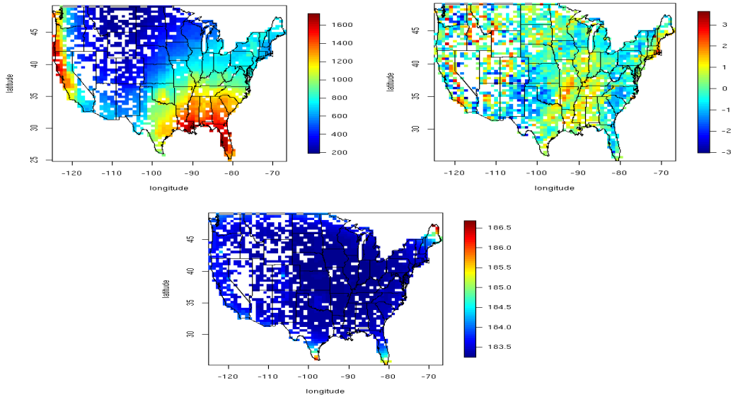
FIG 5. Cubic Model in Lat and Lon including Elevation: Fitted return values (top left), residuals (top right), and prediction standard errors (bottom) from the cubic regression model with NCEP grid data. Errors range between 183.2 and 186.7 tenths of a mm.
