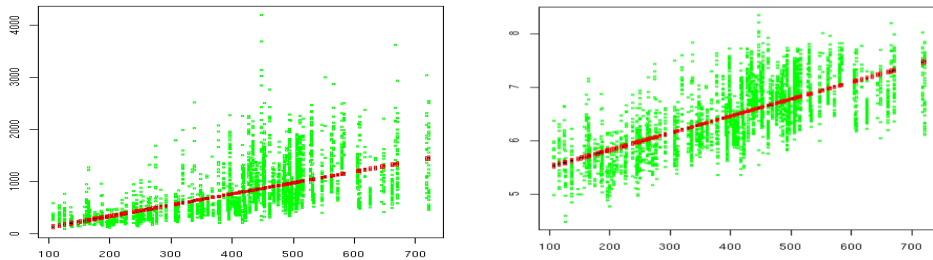
FIG 3. Modeling Point Station Return Values: 100-year return values: point-station returns regressed on gridded return values (left) and log-transform of point-station values regressed on gridded returns (right) for the NCEP grid cell data. Return values are in 10^h s of a millimeter for the winter (DJF) season.
