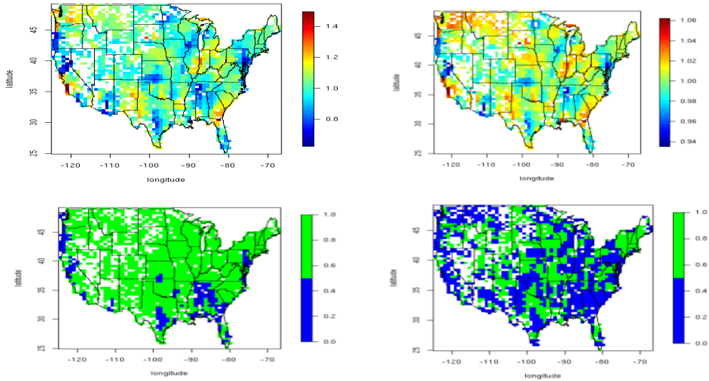
FIG 7. Ratio Future to Present Return Levels: Ratio of predicted point-level return values for the future run (2070-2099) to the predicted point-level return values for the control run (1970-1999) for the CCSM grid cell data (top left). Ratio of the cubic model outputs (top right). Indicator of stations where ratio is significantly different from 1.0 (0.05 level). Bottom left shows the indicators of the scaled return value ratios, bottom right shows indicators of log-scale ratio. “1” (green) indicates no significant difference, “0” (blue) indicates ratio is significantly different from 1.0.
