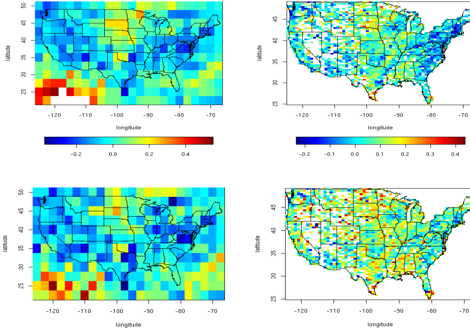
FIG 3. GEV Parameter Estimates: \xi : Comparison of GEV parameter estimates ( \xi ) for both NCEP grid cells (left column) and NCDC point-level (right column) over both 95 th (top row) and 97 th (bottom row) percentile threshold choices.
