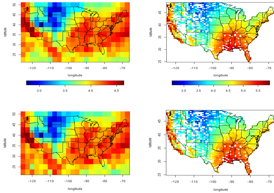
FIG 2. GEV Parameter Estimates: \log(\psi) : Comparison of GEV parameter estimates ( \log(\psi) ) for both NCEP grid cells (left column) and NCDC point-level (right column) over both 95 th (top row) and 97 th (bottom row) percentile threshold choices.
