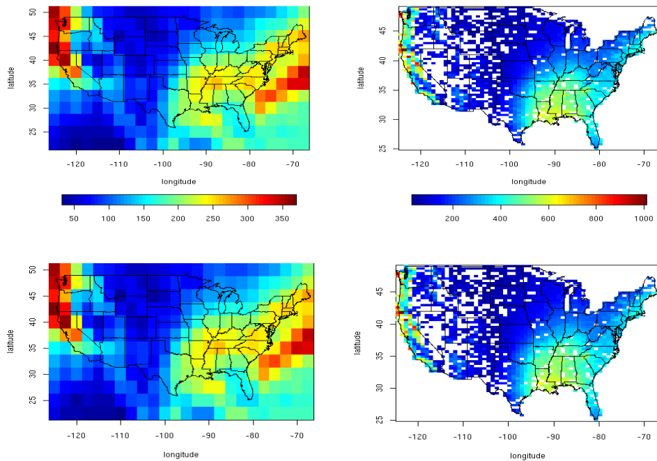
FIG 1. GEV Parameter Estimates: \mu : Comparison of GEV parameter estimates ( \mu ) for both NCEP grid cells (left column) and NCDC point-level (right column) over both 95 th (top row) and 97 th (bottom row) percentile threshold choices.
