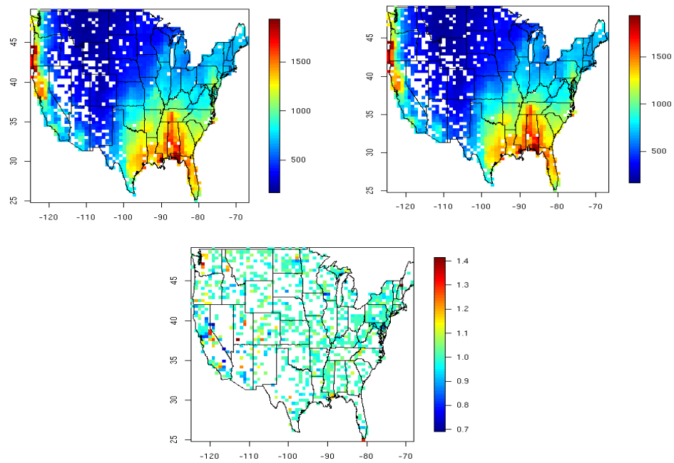
FIG 5. Kriged vs Regression: Comparison of cubic regression model predictions (top) to kriged predictions (center) and the ratio of kriged to regression model predictions for the CCSM grid cell data. Ratio considered for stations un-used in original analysis due to missing values or non-convergence.
